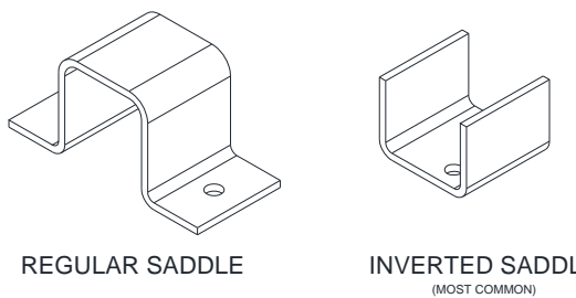
Figure 5.6 – Tube Saddles
