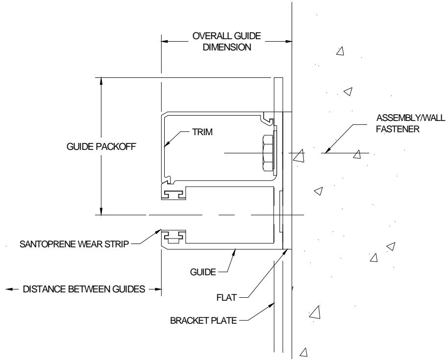
Figure 5.9 – Between Jambs with Back-Up Flat
