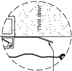
TIEBACK STRAP MOUNT BY CORNELL. (TYP. ON BOTH SIDES OF DOOR)
